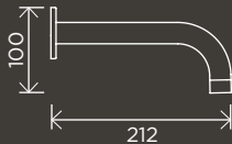
Round Curved Spout
