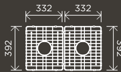
Lavello Protection Grid for MKSP-D1160440D (2pcs)
