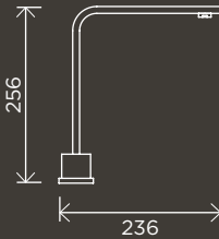
Square High-Rise Swivel Hob Spout
