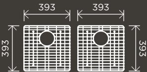
Lavello Protection Grid for MKSP-D860440 (2pcs)
