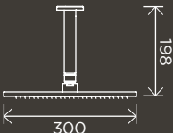
Square Ceiling Shower 300mm Rose, 200mm Dropper
