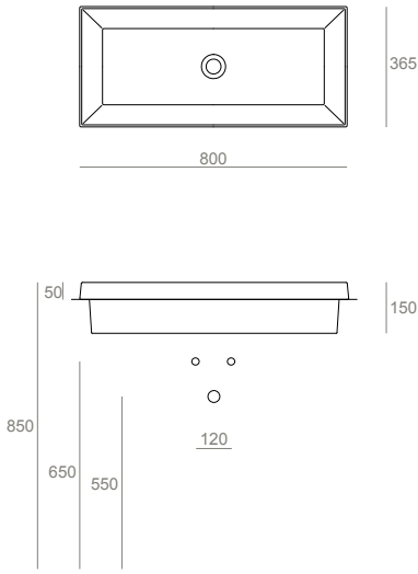
AG80IN Lavabo 80 da incasso. 4 lati smaltati Fully-inset washbasin 80. 4 sides enamelled 80.36,5.15
