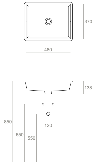
S59 Lavabo 48 sottopiano Undercoat washbasin 48 48.37.14
