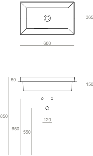
AG60IN Lavabo 60 da incasso. 4 lati smaltati Fully-inset washbasin 60. 4 sides enamelled 60.36,5.15
