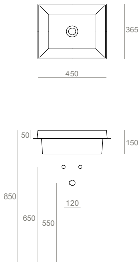
AG45IN Lavabo 45 da incasso. 4 lati smaltati Fully-inset washbasin 45. 4 sides enamelled 45.36,5.15
