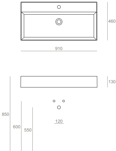
AG91 Lavabo 91 monoforo da appoggio o sospeso Countertop or wall-hung washbasin 91 for single tap hole 91.46.13
