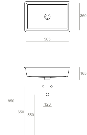
S60 Lavabo 55 sottopiano Undercoat washbasin 55 55.35.16
