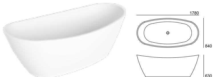
Star Banheira . Bañera . Bathtub . Baignoire 51100201
